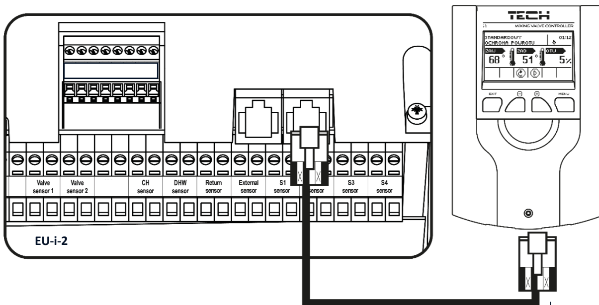
Example connection between additional valve and EU-i-2 main controller
