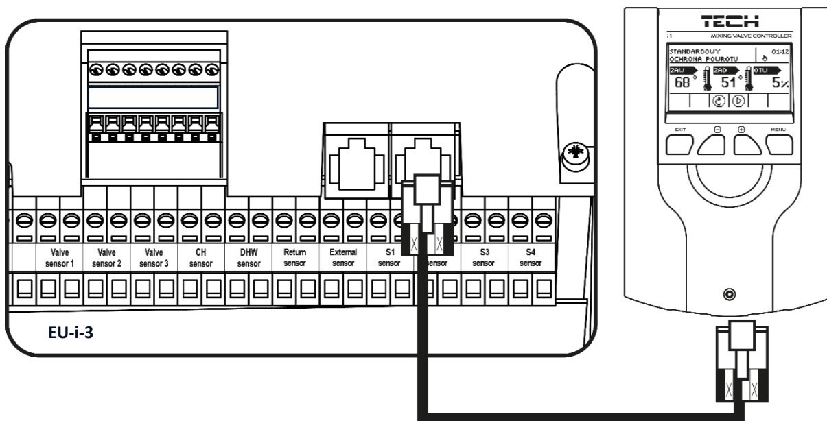
Example connection between additional valve and EU-i-3 main controller
