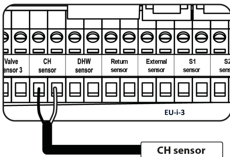
Connecting CH sensor
