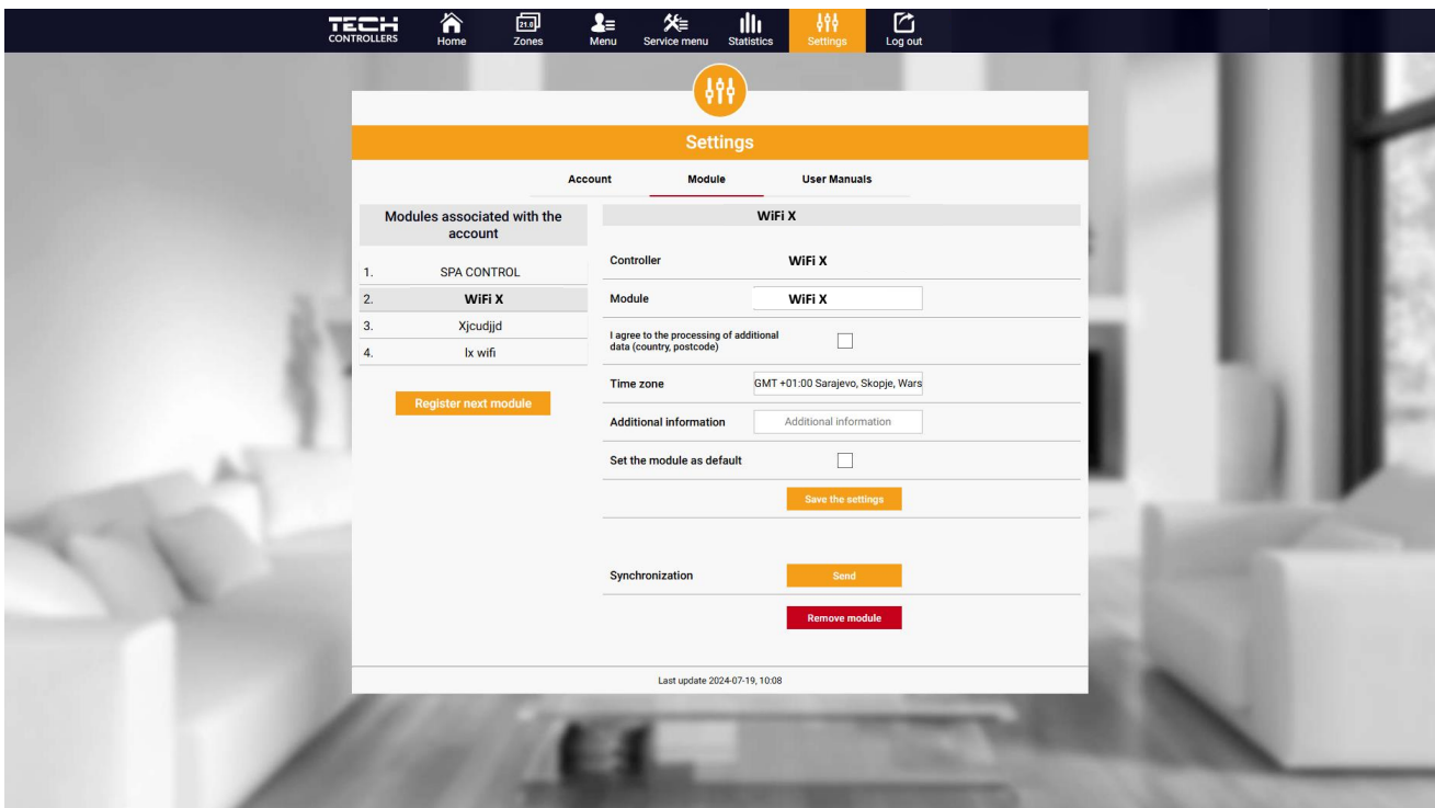
Settings/Module tab
